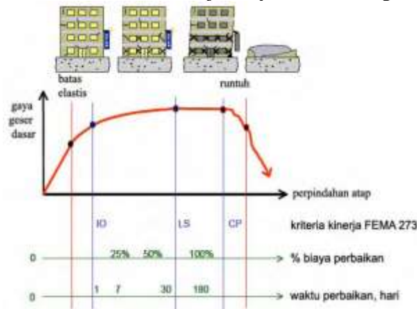
Gambar 1. Ilustrasi Performance Level Sumber: Dewobroto, 2007
