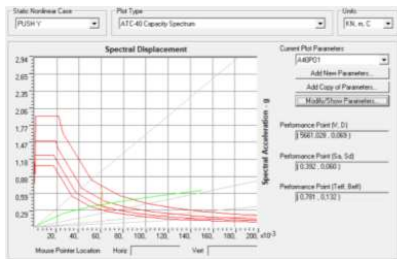
Gambar 7. Capacity spectrum ATC-40 arah Y
