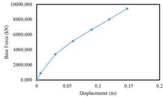
Gambar 5. Kurva pushover arah X
