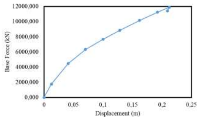
Gambar 4. Kurva pushover arah Y
