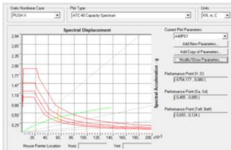
Gambar 6. Capacity spectrum ATC-40 arah X
